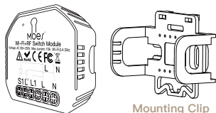
Mounting Clip
